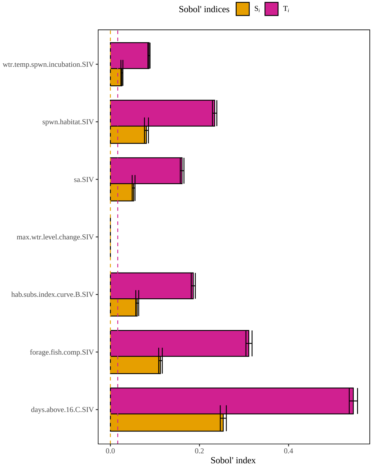
Figure 7. Results of a sensitivity analysis for the whitebassLacCurveBSubsIndex model based on a multiplicative mean structure. Dashed lines represent baseline numerical approximation error for S_i and T_i ( i.e. , dummy variables).
