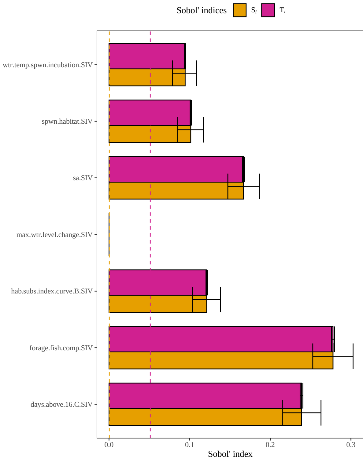
Figure 4. Results of a sensitivity analysis for the whitebassLacCurveBSubsIndex model based on an arithmetic mean structure. Dashed lines represent baseline numerical approximation error for S_i and T_i ( i.e. , dummy variables).
